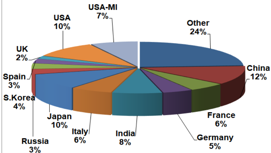
The LISE++ code geography (last 2019 year)
