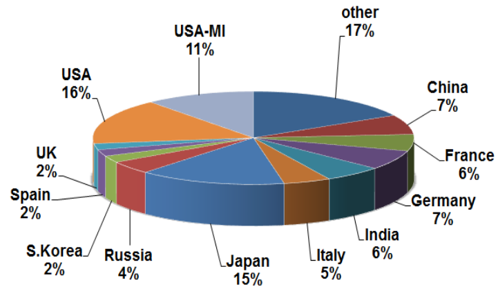
The LISE++ code geography
