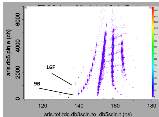
Figure 48: Example of an unbound nucleus PID ( {}^9\text{B} and {}^{16}\text{F} ).
