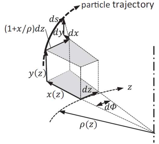
Figure 37: The curvilinear coordinate system used in the definition of the ion optical vector \vec{V} . The optical axis is \vec{s} .
