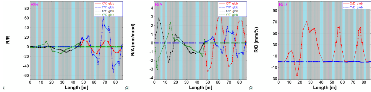
Figure 40: Ideal first-order optics of the k3CB2 mode of ARIS. The plotted quantities represent global transfer matrix elements as a function of position along the beamline. The rotation of the dispersive plane following the pre-separator is clearly visible.
