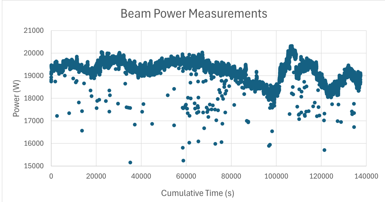
Figure 21: Resulting beam power graph from the beam integral workbook (Figure 20). A trapezoidal integration of this curve yields the total energy delivered to the target.
