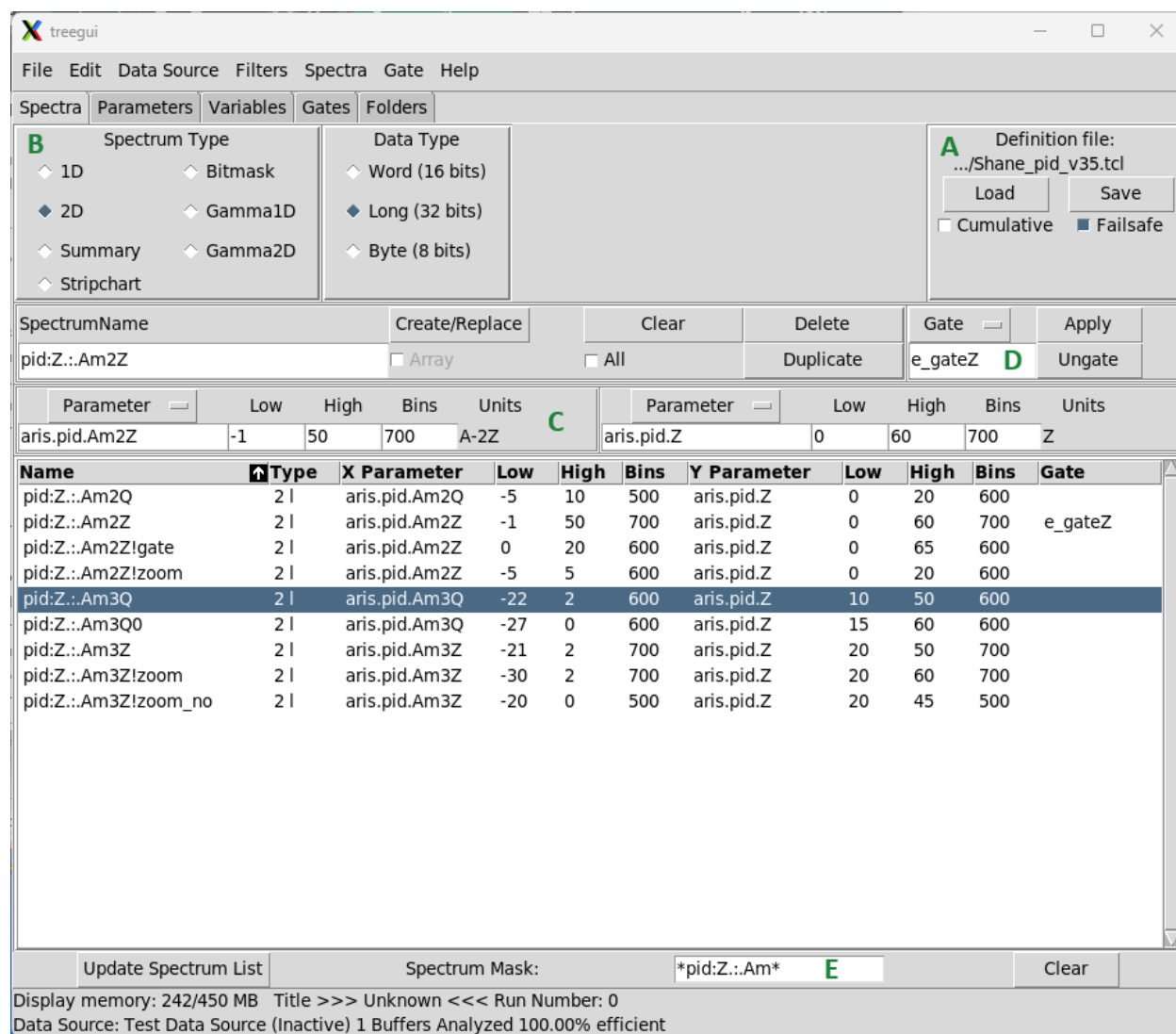
Figure 34: The SpecTcl treegui Spectrum tab interface.
