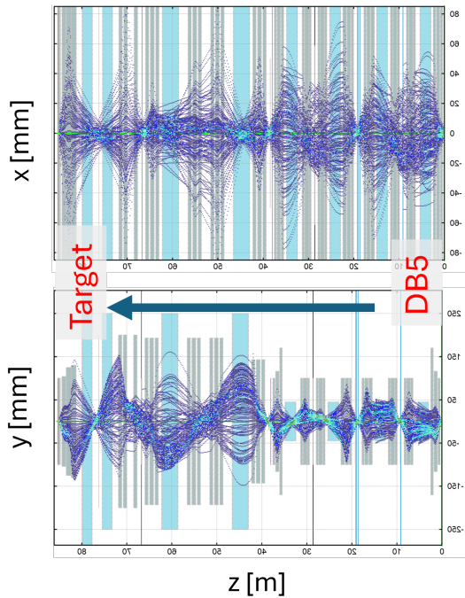
Figure 43: Calculations of particle trajectories traced backward from DB5 to the target position.
