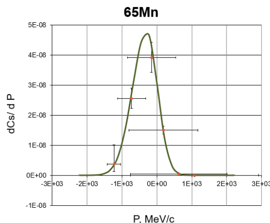
Figure 53: Example of a fitted momentum distribution from six partial cross section measurements.
