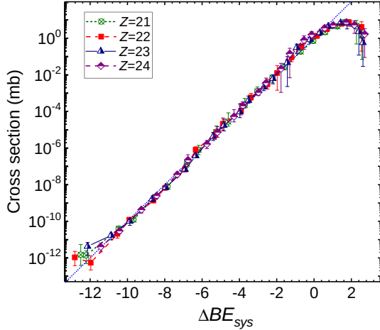
Figure 33: Measured cross sections for isotopes produced in the fragmentation of ^{82}\text{Se} plotted as a function of \Delta BE using the HFB-22 mass table. The blue dotted line represents the fitted functional form \sigma = 10^{\Delta BE_{\text{sys}}} . From Ref. [5].
