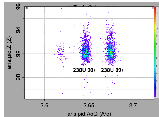
Figure 51: Example of detector calibration and PID using the charge-states of the primary beam ( ^{238}\text{U} ).
