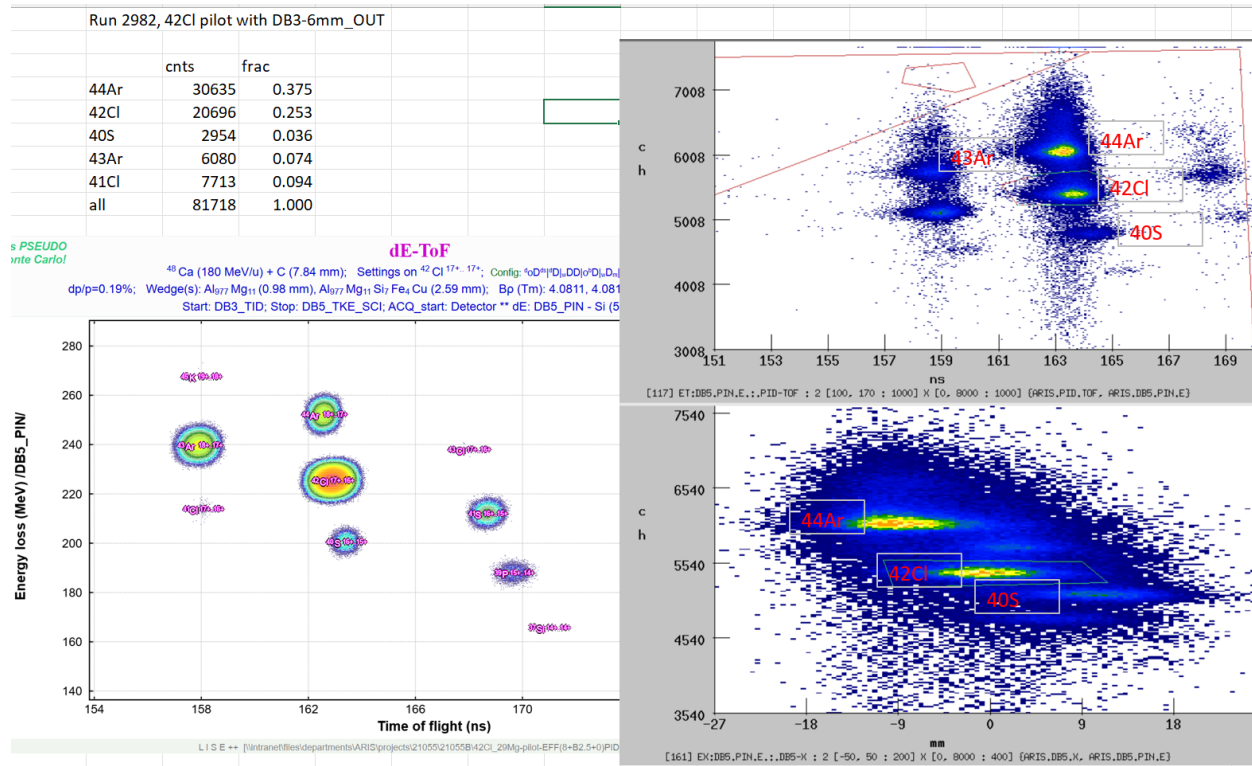
Figure 52: Example of a qualitative comparison of experimental yield to LISE ++ -predicted yield.
