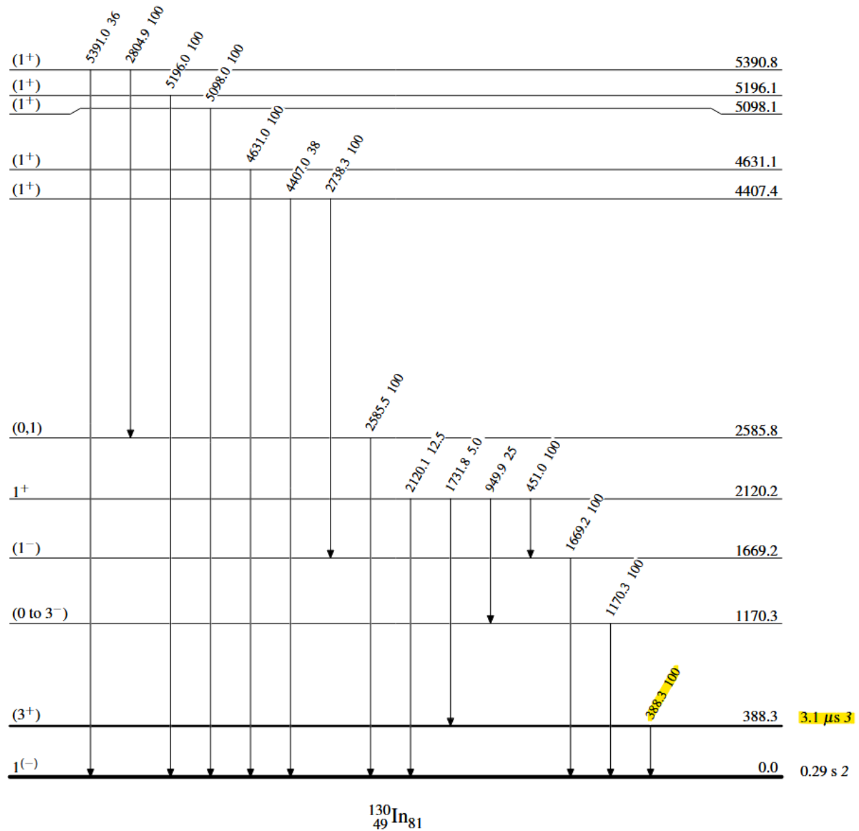
Figure 50: ^{130}\text{In} gamma-ray level scheme from the NNDC ENSDF. The detected isomeric state is highlighted.
