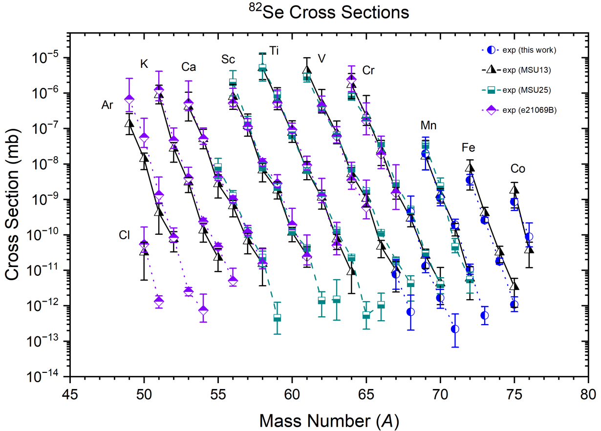
Figure 26: Cross sections from multiple experiments plotted together. From the reaction ^{82}\text{Se} on carbon. Data from Refs. [5, 12] and manuscript in preparation.
