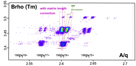
Figure 45: ^{198}\text{Pt} charge-states plotted as a function of A/q and B\rho during a momentum scan in CB1 mode. Prior to trajectory reconstruction, an unphysical correlation is observed.
