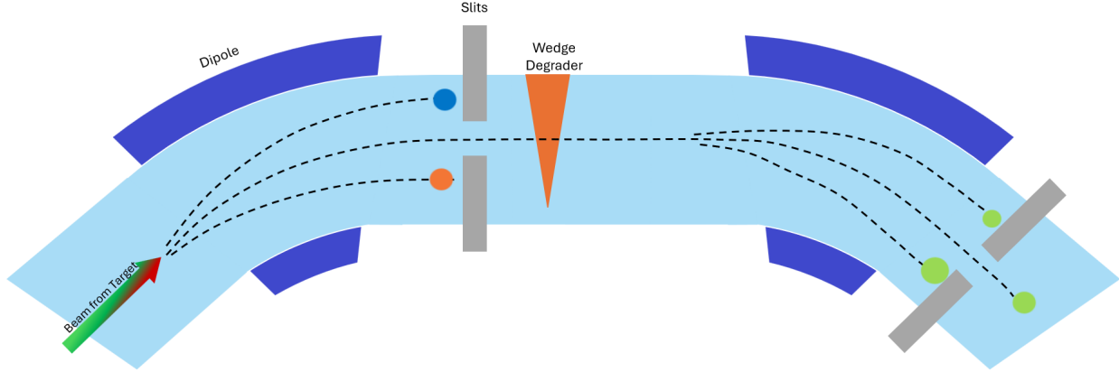
Figure 42: Schematic illustration of secondary beam purification using a wedge degrader between two dipole magnets. This demonstrates the combined action of optical ( B\rho ) and physical (energy-loss) selection lines shown in Figure 41.
