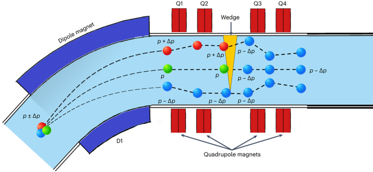
Figure 39: Schematic overview of momentum compression. Identical particles with different initial momenta (color scheme) are spatially separated at a dispersive focal plane and pass through a wedge-shaped degrader, resulting in a reduced momentum spread downstream. Paths of the particles are traced through the system. Taken from Ref. [31].
