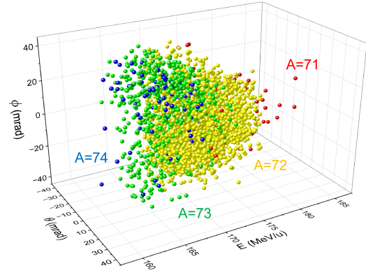
Figure 44: Reconstructed distributions of iron fragments at the target position as a function of energy and transverse angles.
