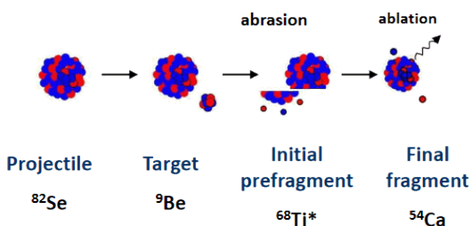
Figure 27: Schematic illustration of the abrasion–ablation process.
