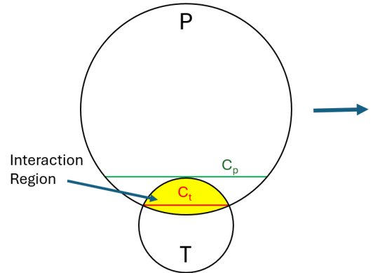
Figure 28: Geometry of a simple abrasion-ablation model at maximum overlap. The chords used for a simple friction calculation are shown.
