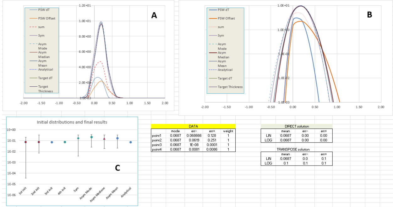
Figure 25: Transmission uncertainty components for ^{67}\text{Cr} (parameter indices 1–4) and the final combined transmission uncertainty for various methods.
