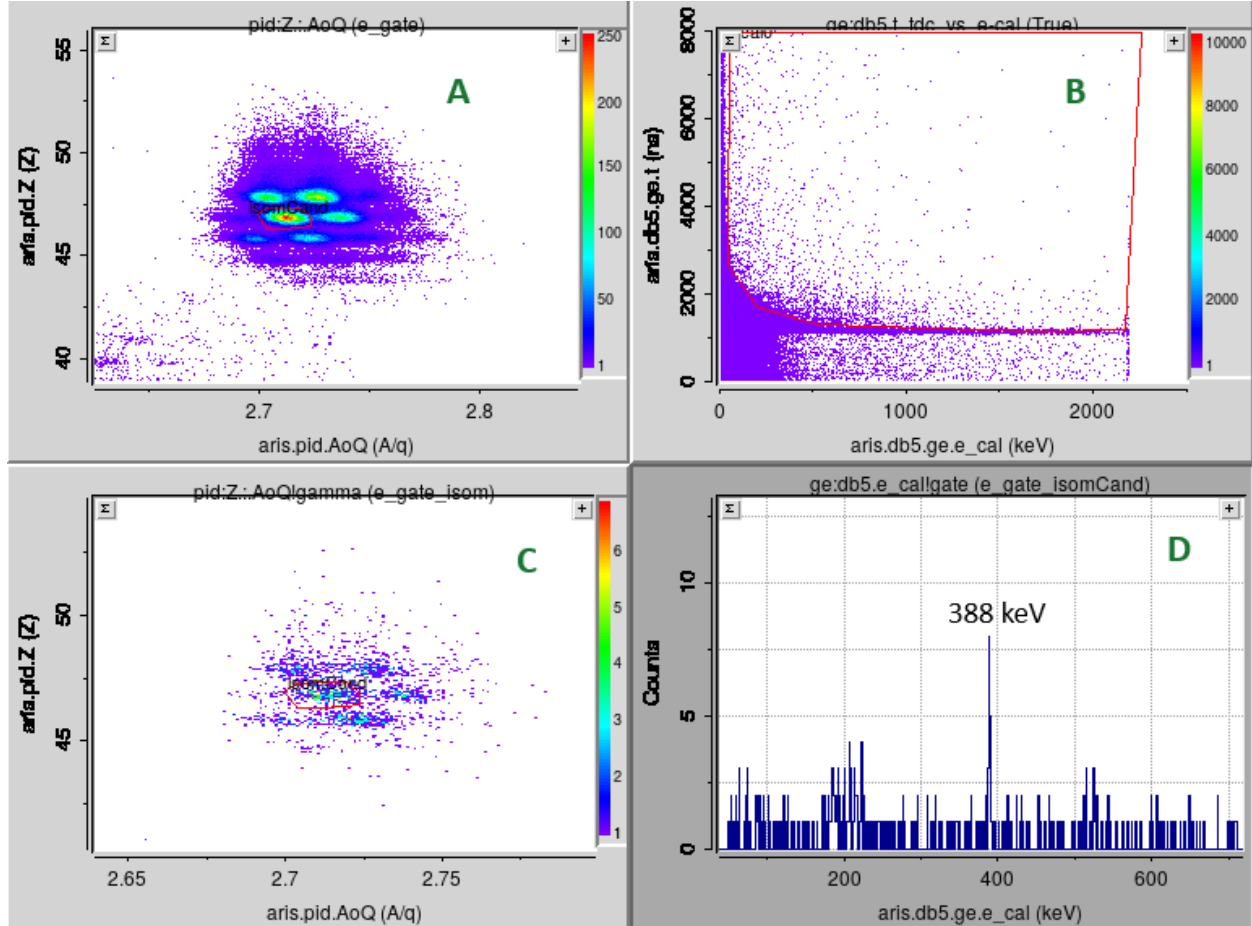
Figure 49: Example of the isomer PID process. Clockwise from top left: (A) finalized and cleaned PID. (B) Germanium detector's registered energy vs time. (C) Isomer gate projected onto PID spectrum. (D) One-dimensional \gamma -energy spectrum with cleaning and blob gate applied.
