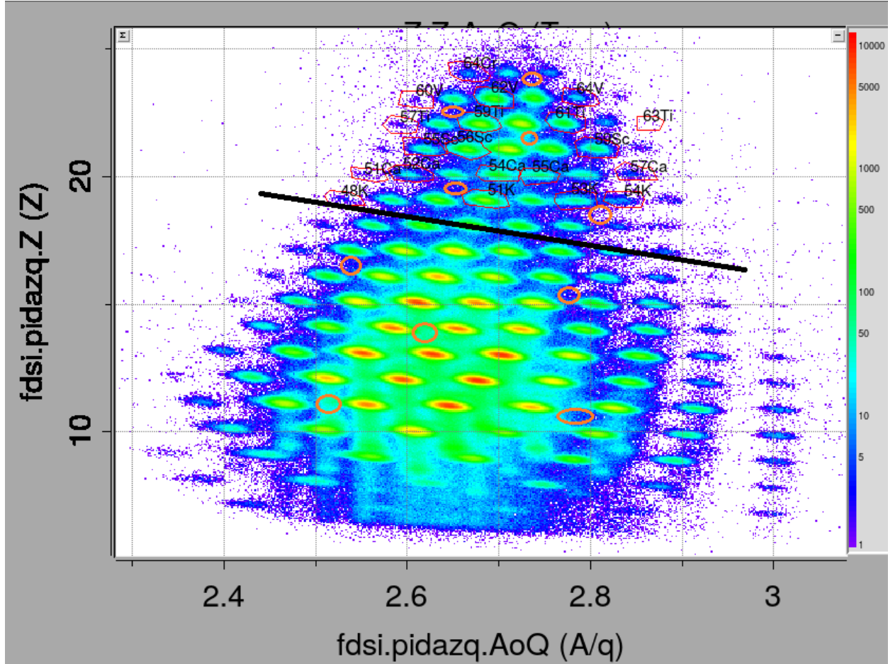
Figure 47: Final calibrated PID spectrum with fragment-identification gates and between-blob (“bad region”) gates defined. Orange circles indicate regions between isotope blobs used to quantify background suppression. The black line separates primary fragments (above) from wedge products and aberration-transported fragments (below).
