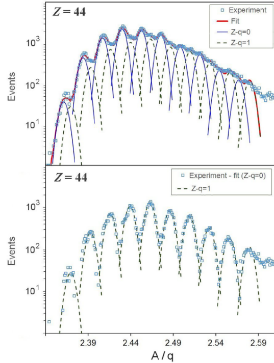
Figure 15: Example of potential charge-state contamination to the yield statistics. From Ref. [6].
