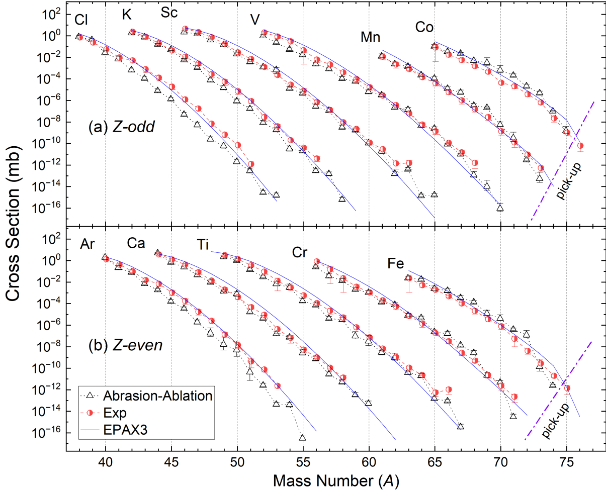
Figure 32: Abrasion-ablation and EPAX3 predicted cross sections vs experimentally measured cross sections. Pick-up reactions are labeled.
