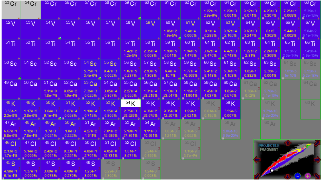
Figure 22: LISE ++ calculations of rate and transmission with secondary and wedge reactions enabled.
