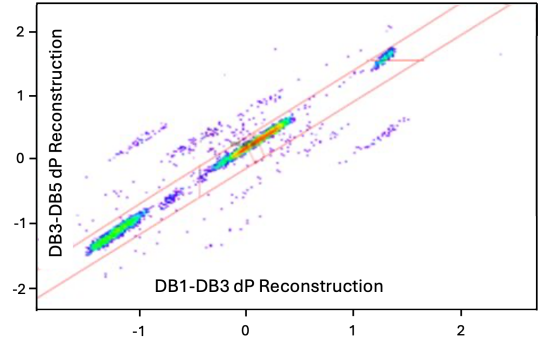
Figure 46: Reconstructed momentum deviations, \Delta B\rho/B\rho , for the DB1-3 and DB3-5 segments of the C-Bend for ^{198}\text{Pt} fragments.
