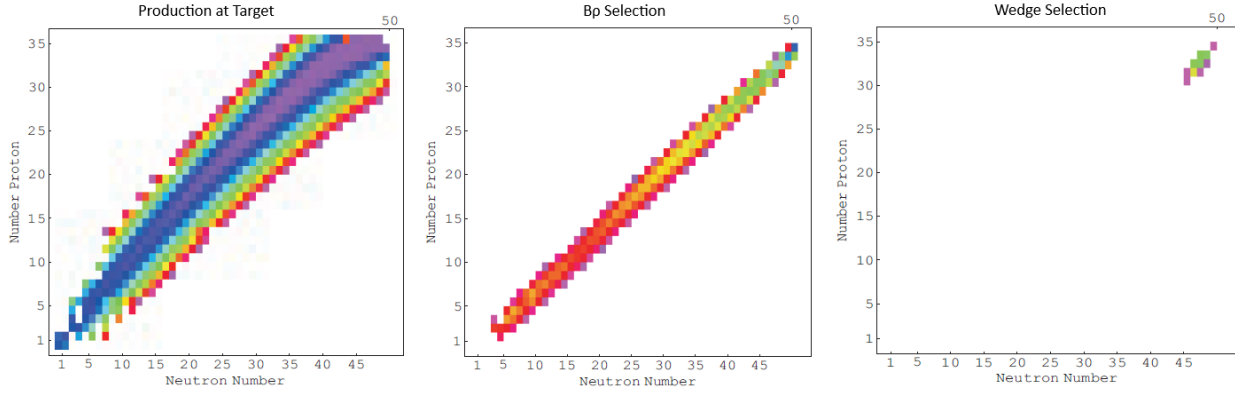
Figure 41: Illustration of selection lines and the resulting increase in beam purity achieved through magnetic rigidity ( B\rho ) selection and energy-loss degradation ( dE ). From Ref. [32]
