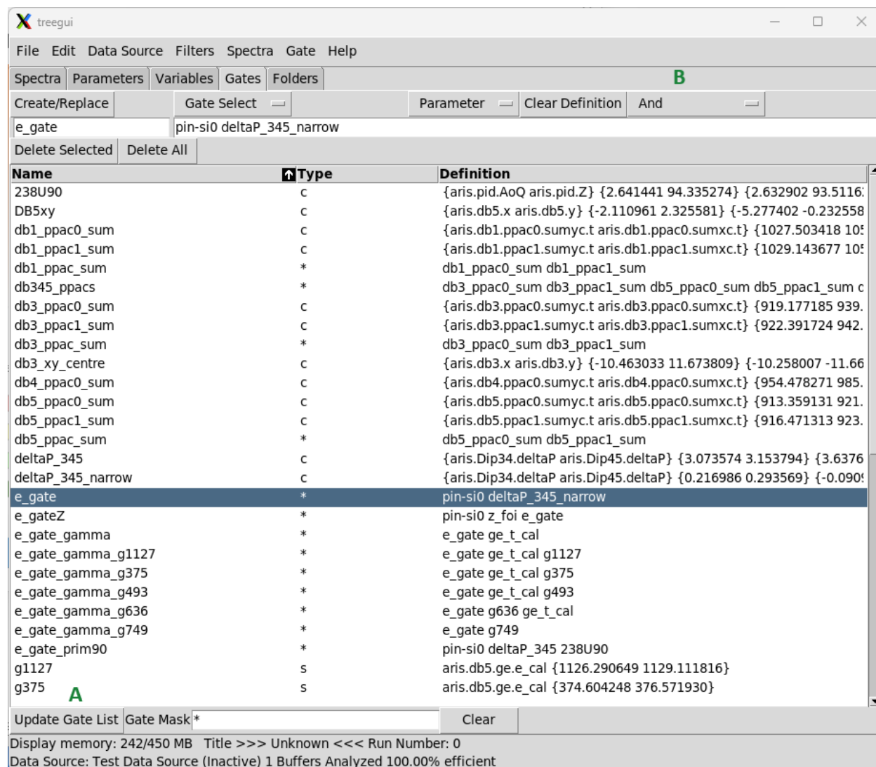
Figure 35: The SpecTcl treegui Gates tab interface.
