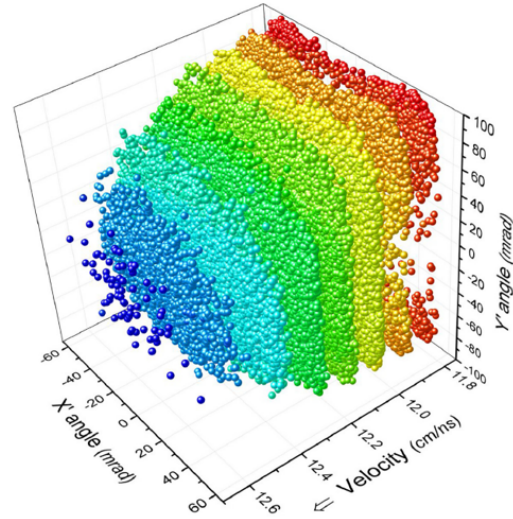
Figure 30: Reconstruction of momentum space as a function of transverse angle of krypton fragments from the fission of uranium. From [6].
